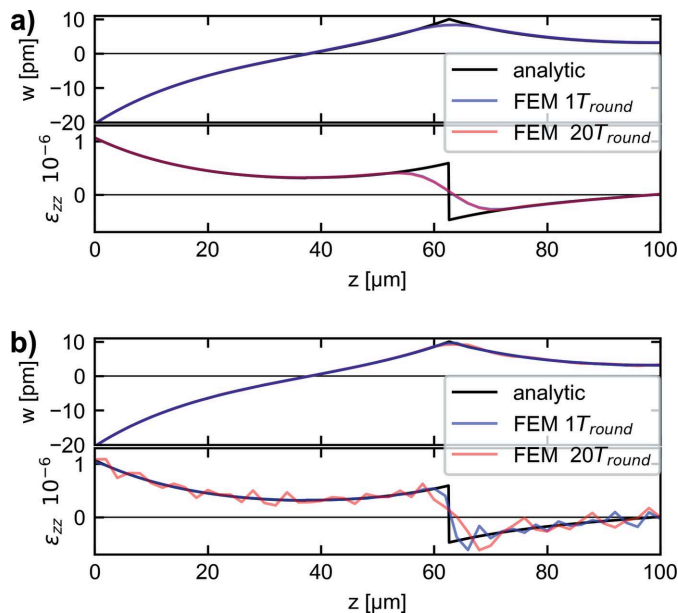
Figure 4 Comparison of analytic solution and FEM solution for displacement w and strain \epsilon_{zz} of a one-dimensional wave at time t = 3.5\ \text{ns} after photon–matter interaction and after t = 3.5\ \text{ns} + 20T_{\text{round}} . (a) Using a temporal Gaussian profile with t_p = 600\ \text{ps} for the FEM simulation. (b) Considering an instantaneously temperature rise at t = 0\ \text{ns} .
