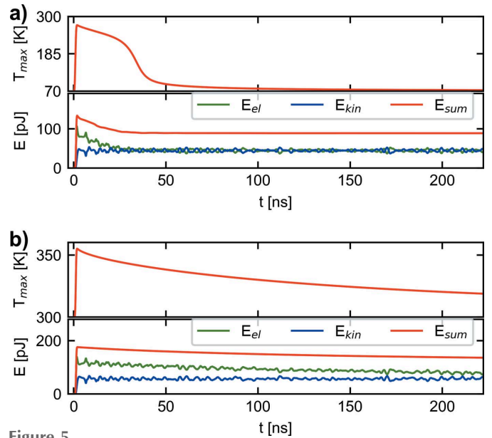
Figure 5 Temporal development of the maximum temperature value and the kinetic and elastic energy, calculated for an initial temperature of (a) T_0 = 70 K and (b) T_0 = 300 K.
